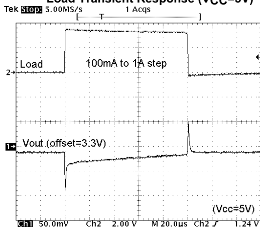
Load Transient Response (VCC=5V)
