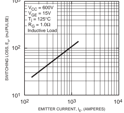
SWITCHING LOSS VS. EMITTER CURRENT (TYPICAL)
