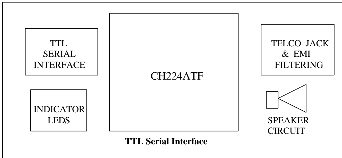
CH224ATF Integrated System Block Diagram
