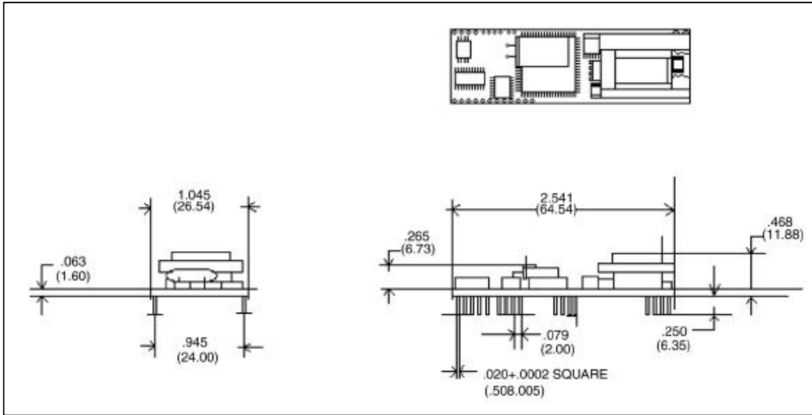
Figure 5. CH224ATF Physical Dimensions
