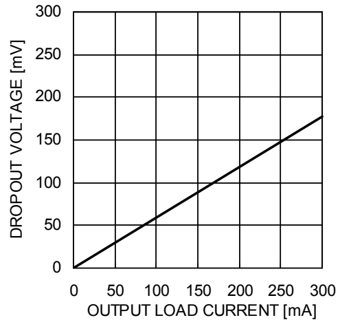
Dropout vs. Load Current
