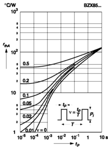
Pulse thermal resistance versus pulse duration Valid provided that leads are kept at ambient temperature at a distance of 10 mm from case.
