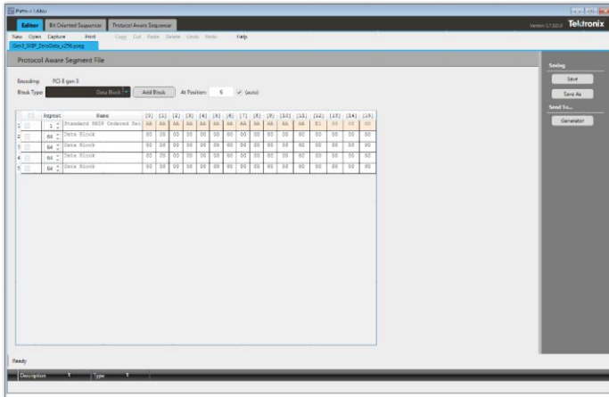
Sequence editor
