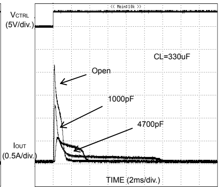
Fig.53 Inrush current vs. Ccss (BD6522F)
