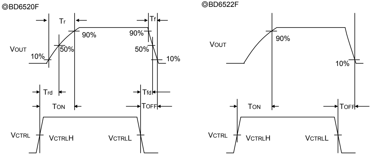
Fig.2 Timing diagram
