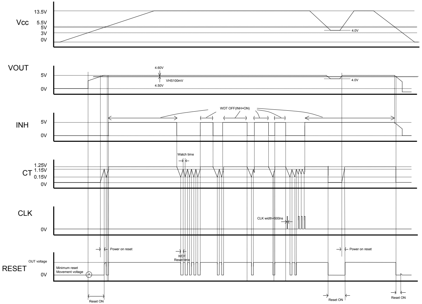
<Timing Chart>
