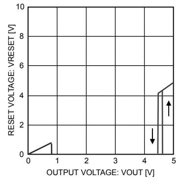
Fig.9 Restion Voltage (Vcc=VOUT)
