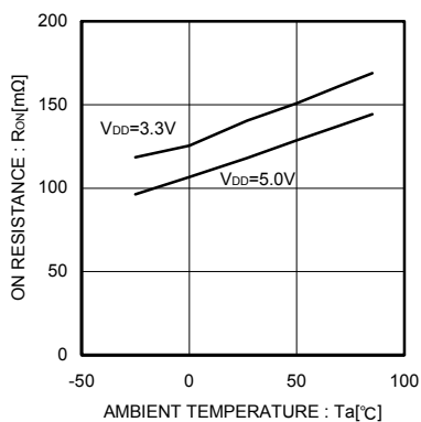
Fig.32 ON resistance
