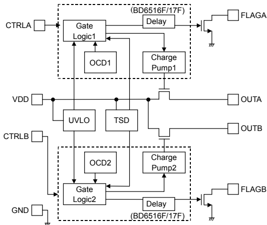
Fig.83 Block diagram
