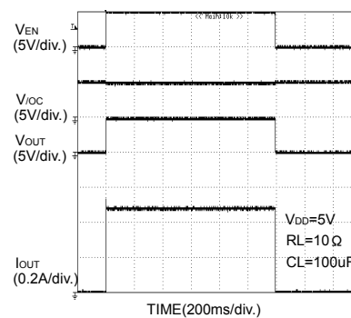
Fig.73 Output rise, fall characteristic (BD2052AFJ)
