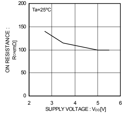
Fig.57 ON resistance
