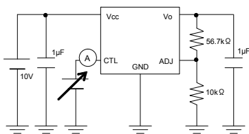
Measurement Circuit of Fig.10
