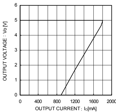
Fig.5 Load Regulation
