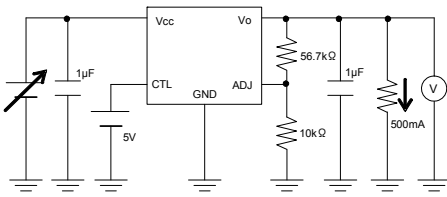
Measurement Circuit of Fig.4
