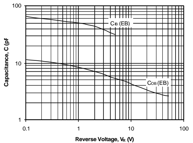
Fig. 4. Typical Capacitances
