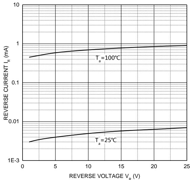
Reverse Characteristics
