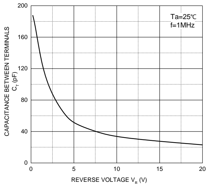
Capacitance Characteristics
