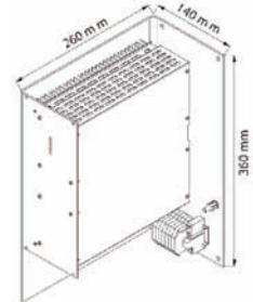
Wall mount / approx. 8.0 kg
