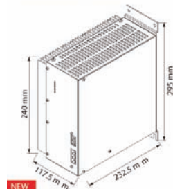
NEW Chassis mount / approx. 5.5 kg
