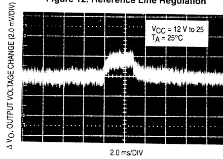
Figure 12. Reference Line Regulation
