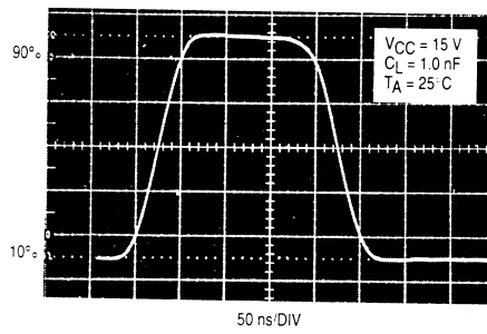
Figure 14. Output Waveform
