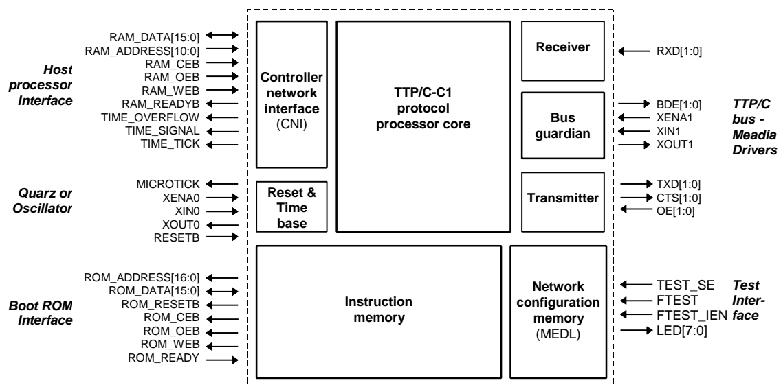
Figure 1 Block Diagramm
