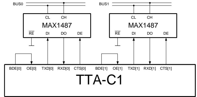
Figure 8: Transceivers with Three-State Output
