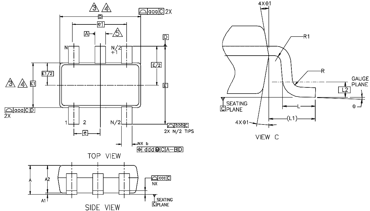
Figure 13. TSOT23-5 Package
