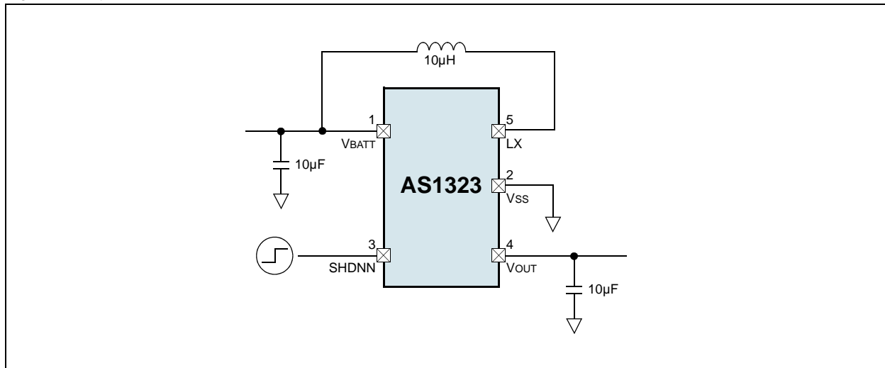
Figure 12. Typical Application
