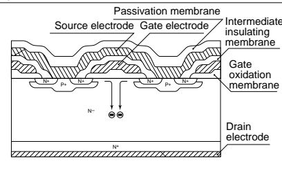
Cross section of the normally-closed type of power MOS
