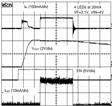
TIME (0.1ms/div)
