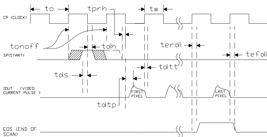
Figure 3: Timing Diagram of the AMIS-720639 Sensor
