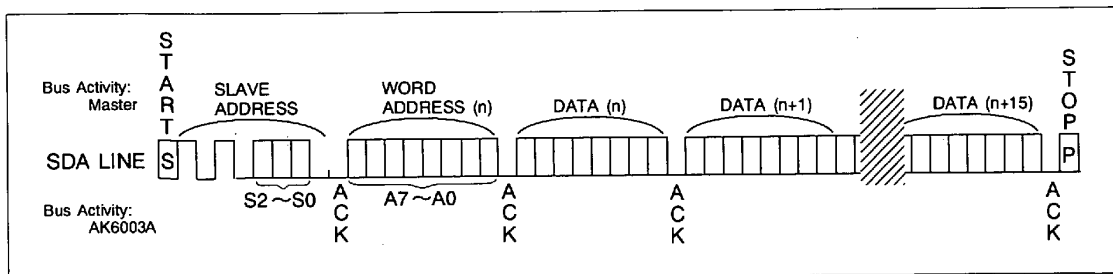
PAGE WRITE
