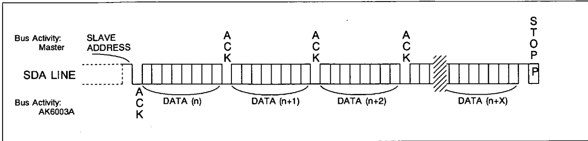
SEQUENTIAL READ
