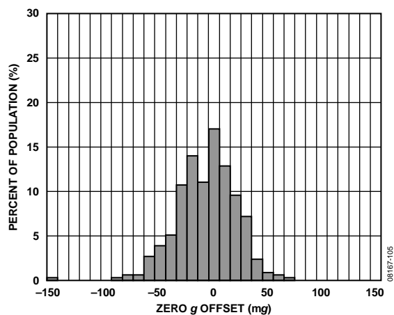
Figure 8. Y-Axis Zero g Offset at 25°C, V_s = 1.8 V
