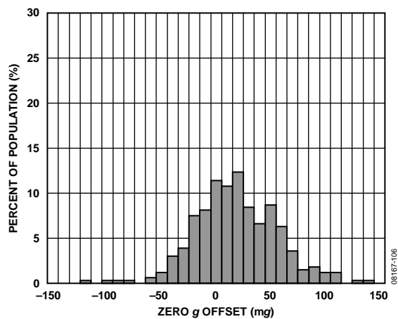
Figure 9. Z-Axis Zero g Offset at 25°C, V_s = 1.8 V
