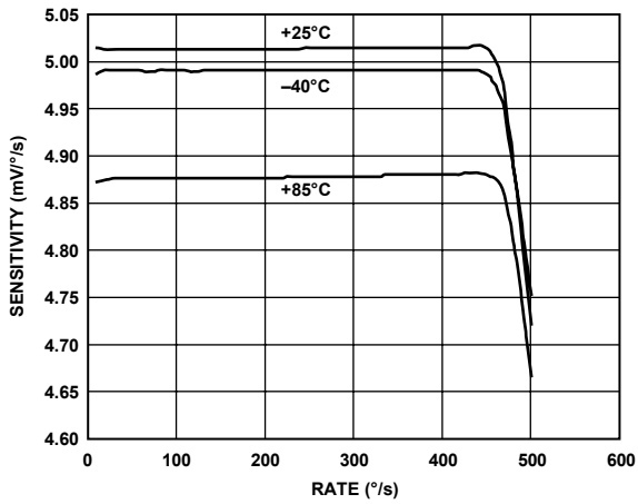
Figure 5. Gain Sensitivity vs. Angular Rate and Temperature, VCC = 5 V
