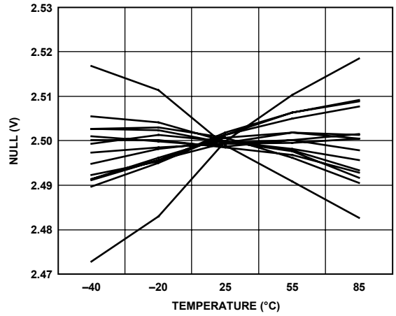
Figure 7. Null vs. Temperature, VCC = 5 V
