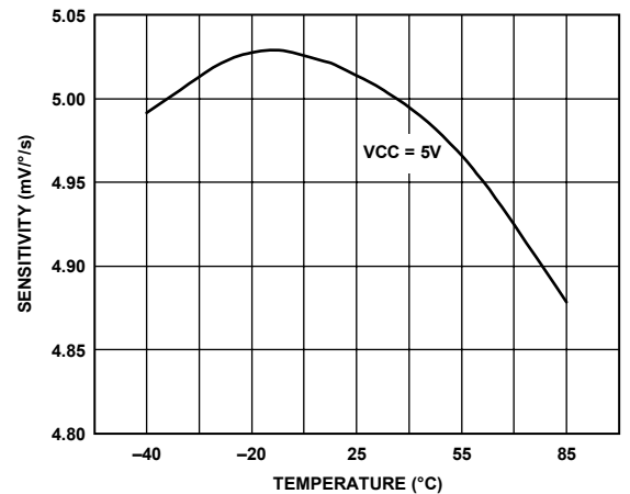
Figure 6. Gain Sensitivity vs. Temperature @ ±300°/sec
