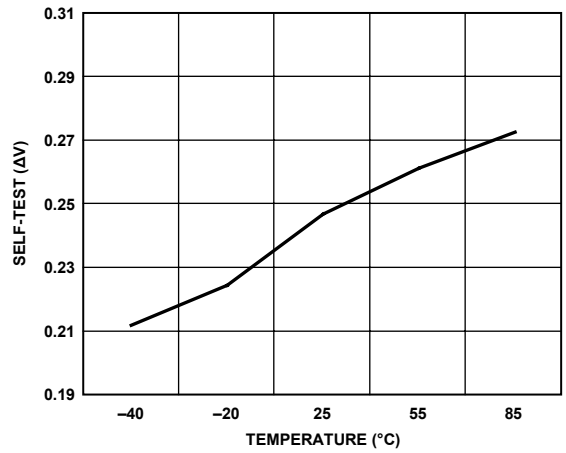
Figure 8. Self-Test vs. Temperature, VCC = 5 V
