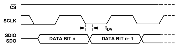
Figure 12. Timing Diagram for Register READ to AD9725
