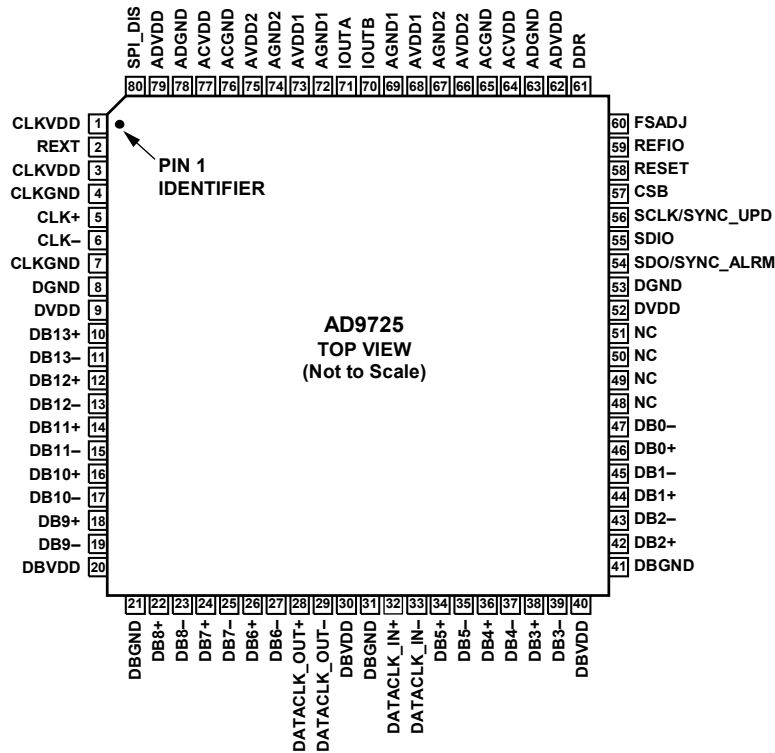
Figure 4. Pin Configuration
