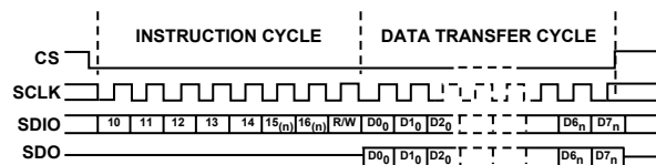
Figure 10. Serial Register Interface Timing LSB First
