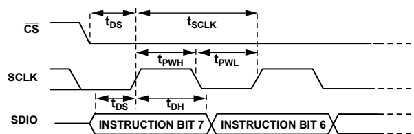
Figure 11. Timing Diagram for Register Write to AD9725
