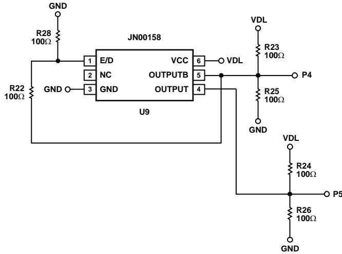
Figure 68. Evaluation Board Schematic—LVDS (continued)
