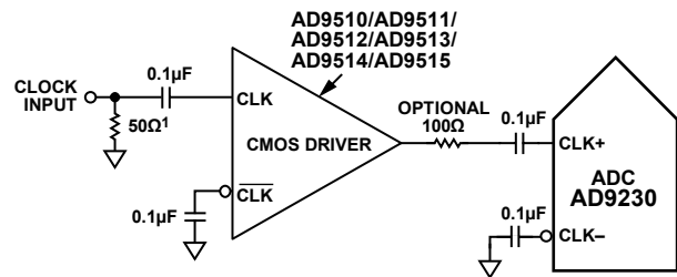
Figure 59. Single-Ended 3.3 V CMOS Sample Clock
