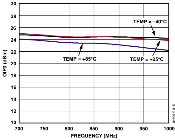
Figure 15. Output IP3 vs. Frequency and Temperature, Maximum Gain, 1 I/O
