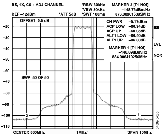
Figure 35. Output Spectrum, Single-Carrier CDMA2000 Test Model at -5 dBm, V_I = V_Q = 0.353 V, ACP Measured at 750 kHz and 1.98 KHz Carrier Offset, Noise Measured at \pm 4 MHz Carrier Offset, Input Signal Filtered Using a Cavity Tuned Filter (Pass Band = 4.6 MHz)
