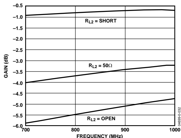
Figure 32. Gain of the AD8340 Using a Single-Ended Output with Different Dummy Loads, R_{L2} on the Unused Output
