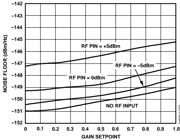
Figure 9. Output Noise Floor vs. Gain, Noise in dBm/Hz, No Carrier, With Carrier (20 MHz Offset) Pin = -5, 0, and +5 dBm
