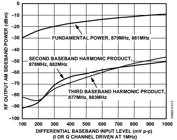
Figure 13. Baseband Harmonic Distortion (I and Q Channel, RF Input = 0 dBm, Balun and Cable Losses of Approximately 2 dB Not Accounted for in Plot)
