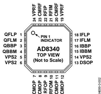
Figure 2. 24-Lead Lead Frame Chip Scale Package (LFCS)
