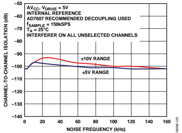
Figure 29. Channel-to-Channel Isolation
