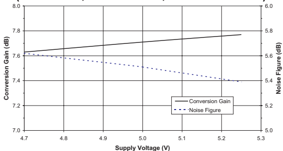
Figure 4: Typical Conversion Gain and Noise Figure vs. Supply Voltage ( T_A = +25\text{ }^\circ\text{C} , f_{RF} = 450\text{ MHz} , f_{IF} = 1087.75\text{ MHz} )
