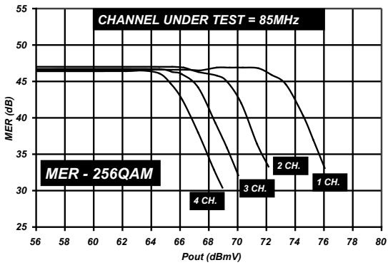
Figure 11: ACA0862B MER - 256 QAM @ 85 MHz
