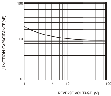
FIG3-TYPICAL JUNCTION CAPACITANCE
