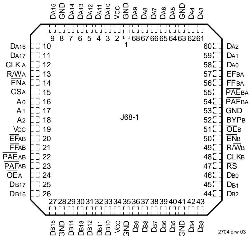
PLCC Top View
