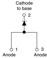
VS-60APU06PbF
