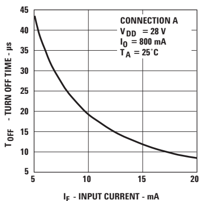
Figure 15. Typical Turn Off Time vs. Input Current.
