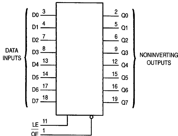
LOGIC DIAGRAM
