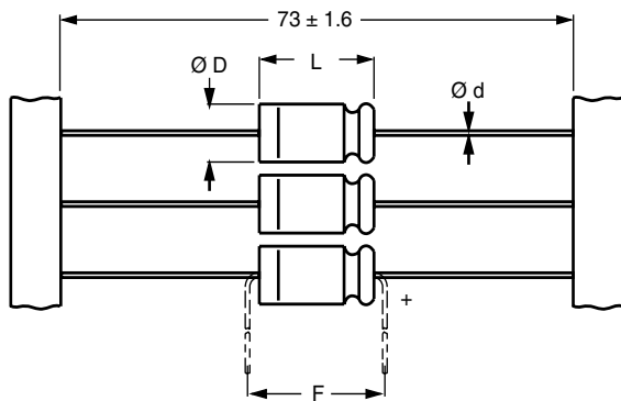
Form BR: Taped on reel case ∅ D x L = 6.5 x 18 to 15 x 30 mm Form BA: Taped in box (ammopack) case ∅ D x L = 6.5 x 18 to 10 x 25 mm
