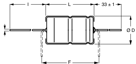
Form AA: Axial in box case ∅ D x L = 10 x 30 to 21 x 38 mm
