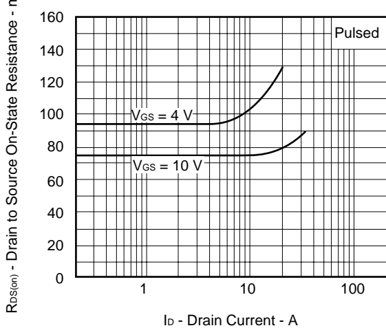
DRAIN TO SOURCE ON-STATE RESITANCE vs. DRAIN CURRENT
