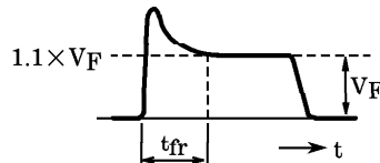
WAVEFORM
