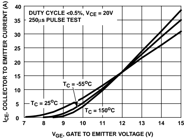
FIGURE 13. TRANSFER CHARACTERISTIC
