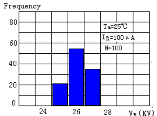
Avalanche Breakdown Voltage Distribution
