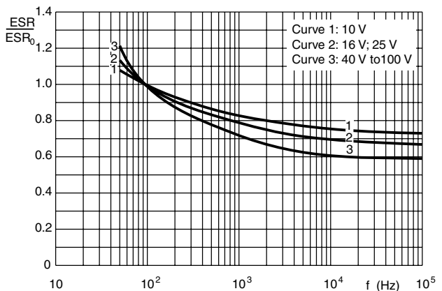
Case Ø D x L = 10 x 30 to 21 x 38 mm ESR 0 = typical at 20 °C, 100 Hz
