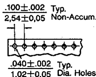
Recommended P.C. Board Layout for .100" (2.54 mm) Headers
