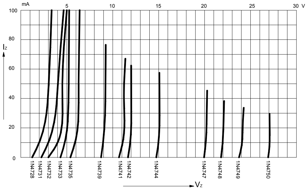
FIG.1 – BREAKDOWN CHARACTERISTICS
