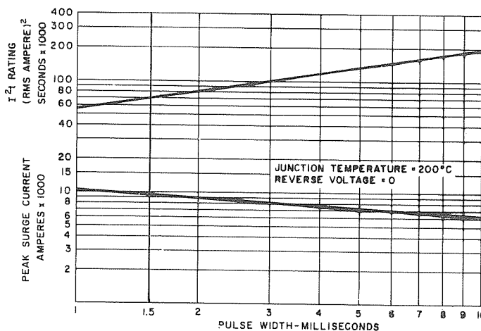
4. SUB-CYCLE SURGE FORWARD CURRENT AND I^2t RATING VS. PULSE TIME FOLLOWING RATED LOAD CONDITIONS
