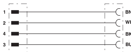
Contact assignment of M12 connector/socket
