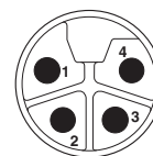
Pin assignment M12 male connector, 4-pos.
