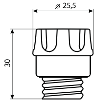
Fuse carrier/cap
