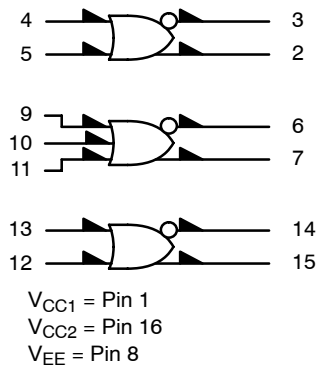
Figure 1. Logic Diagram
