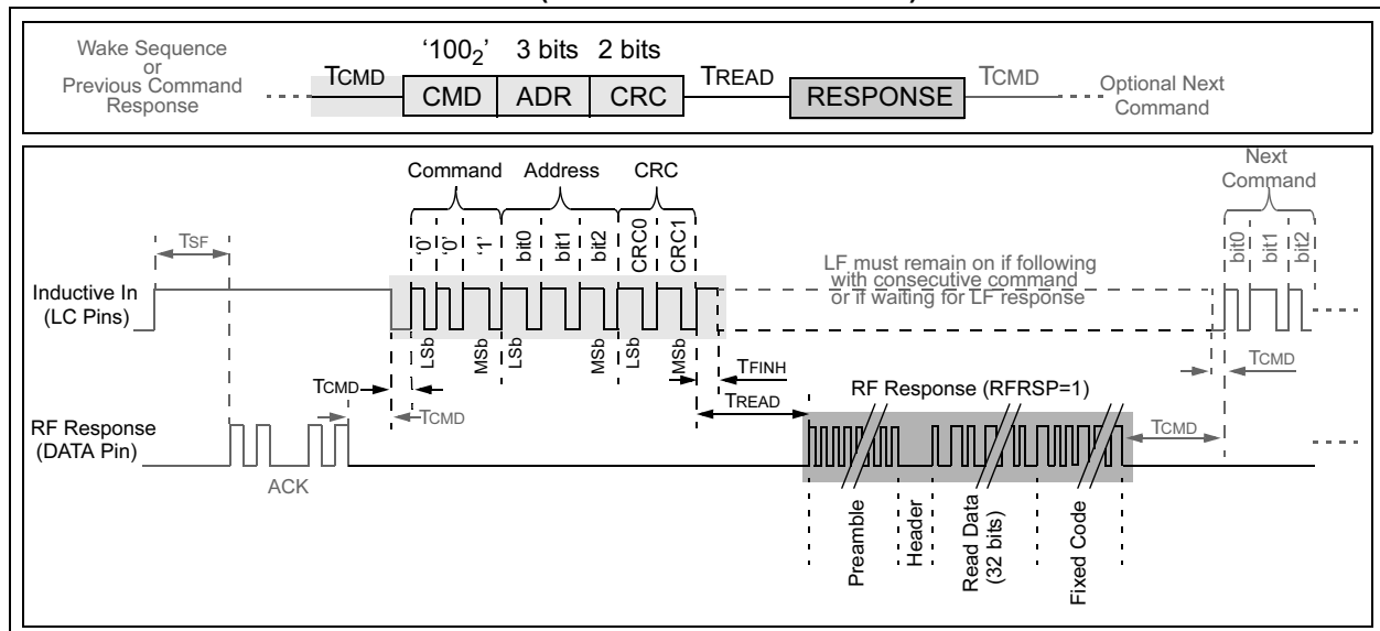
FIGURE 3-15: READ SEQUENCE (RF RESPONSE EXAMPLE)
