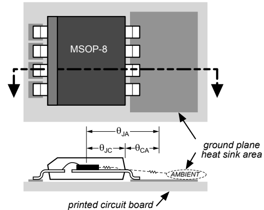
Figure 3. Thermal Resistance
