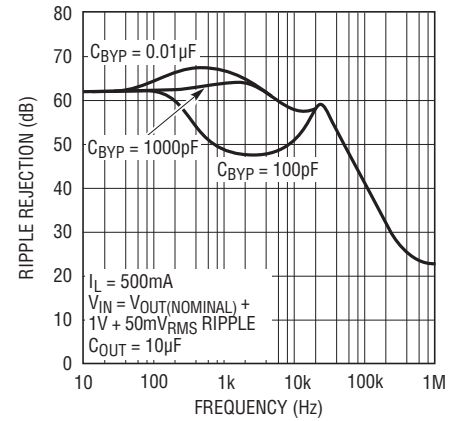
Output 1 Input Ripple Rejection
