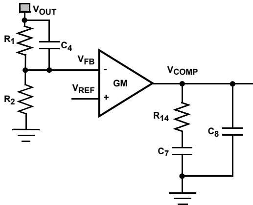
FIGURE 56. TYPE II COMPENSATOR
