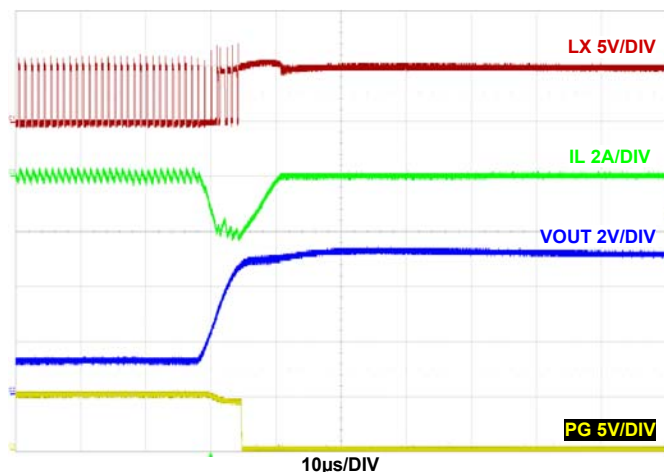
FIGURE 51. OVERT VOLTAGE PROTECTION F_{SW} = 2\text{MHz} , V_{IN} = 5\text{V} , MODE = PFM, T_A = +25^\circ\text{C}
