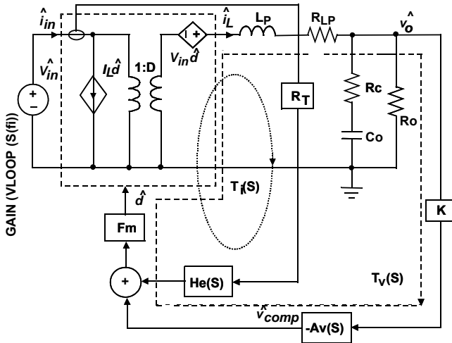
FIGURE 55. SMALL SIGNAL MODEL OF SYNCHRONOUS BUCK REGULATOR
